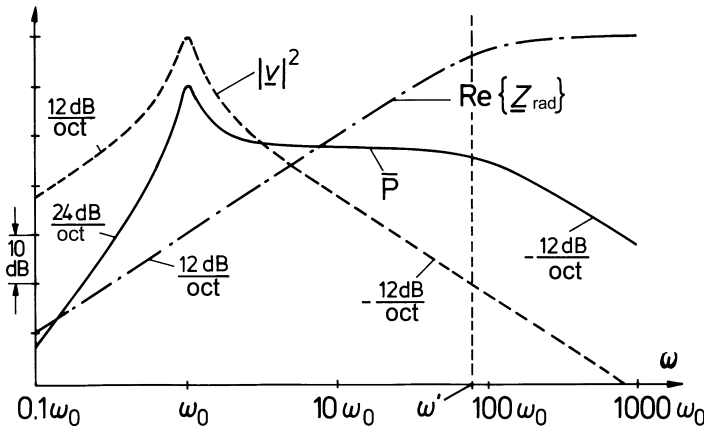
Fig. 5.7. Tuning the frequency response of dynamic loudspeakers
