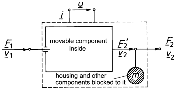
Fig. 4.2. Schematic representation of a coupling element, distinguishing mobile components and components blocked to the housing
