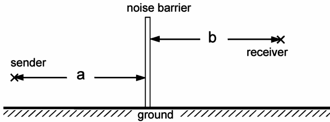
Fig. 15.19. Noise barrier
