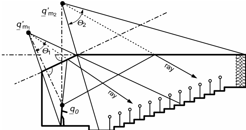
Fig. 12.7. Guiding sound via the ceiling of an auditorium
