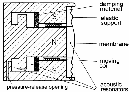
Fig. 5.10. Moving-coil microphone
