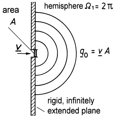
Fig. 10.1. Hemispherical sound field, originating from a point source in a flat and rigid baffle
