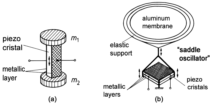
Fig. 6.6. (a) Two-mass longitudinal vibrator, (b) crystal microphone
