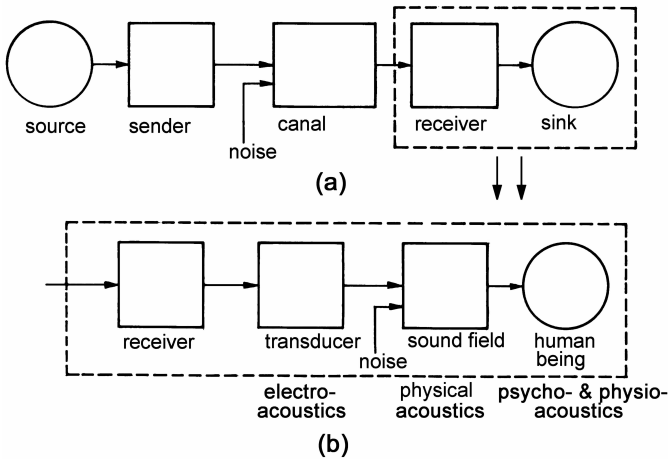
Fig. 1.1. Schematic of a transmission system (a) general, (b) electroacoustic transmission system – receiving end
