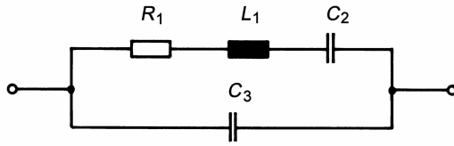
Fig. 15.12. Equivalent circuit of a quartz oscillator
