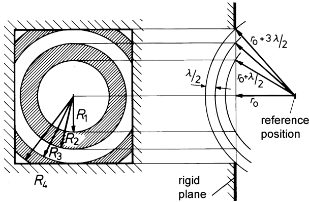
Fig. 10.7. The construction of Huygens-Fresnel zones
