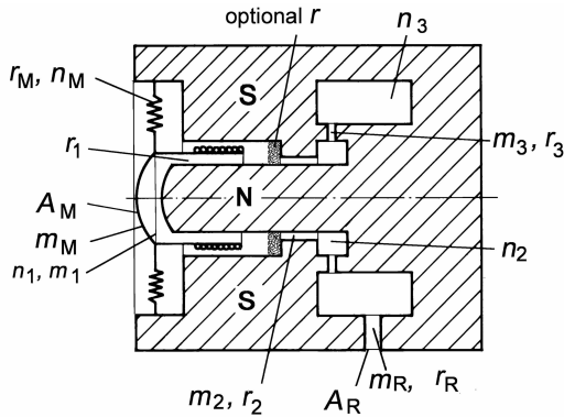
Fig. 15.10. Schematic plot of a moving-coil microphone.
