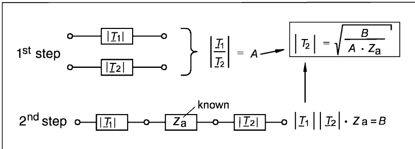
Fig. 4.20. Conceptual summary of the absolute-calibration method
