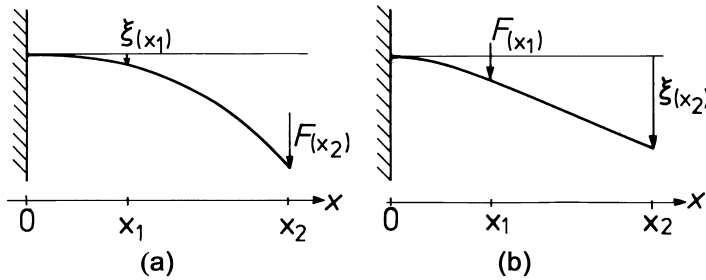
Fig. 4.8. Mechanic reciprocity experiment with a bending beam, (a) Force applied at position x_2 , deflection at position x_1 , (b) vice versa
