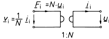
Fig. 4.7. The ideal gyrator as analogy of the ideal electric-field transducer
